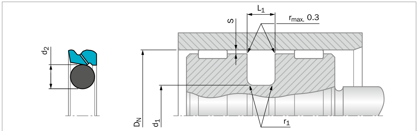
Figure 130: Installation Drawing
