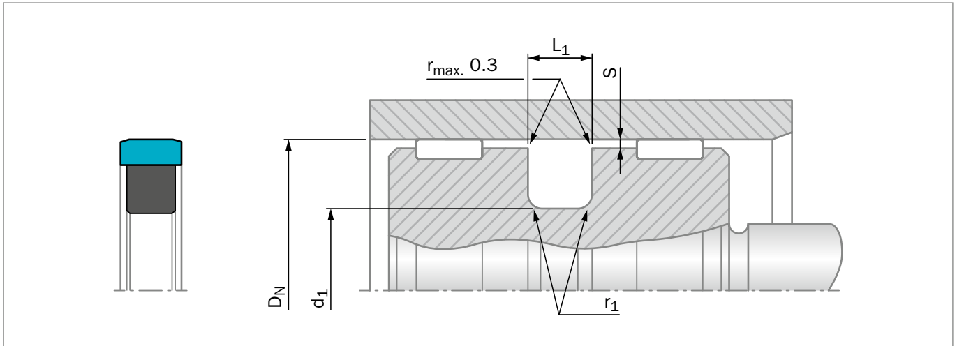
Figure 118: Installation Drawing
