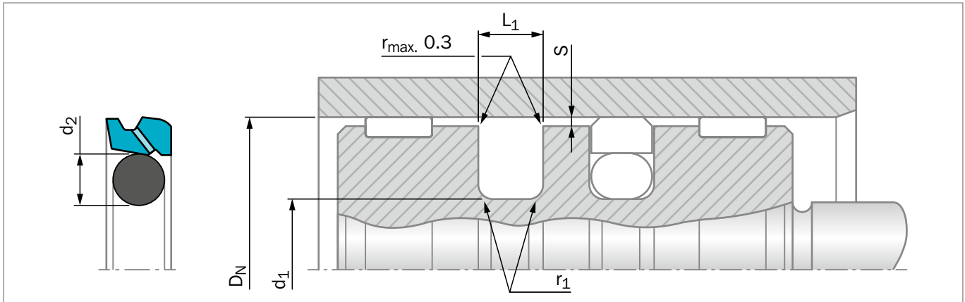
Figure 127: Installation Drawing
