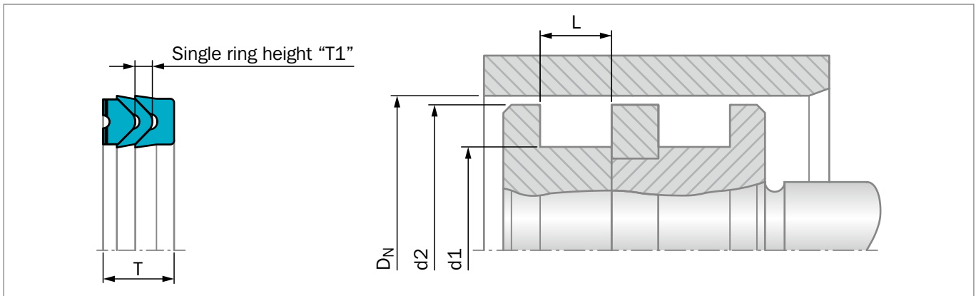
Figure 160: Installation Drawing
