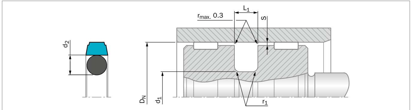
Figure 110: Installation Drawing
