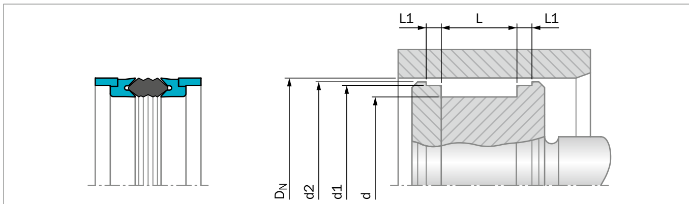
Figure 162: Installation Drawing
