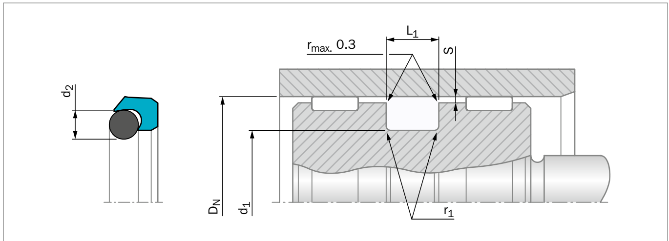
Figure 141: Installation Drawing
